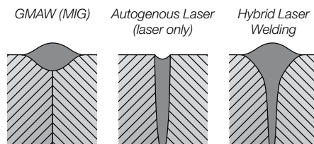
Graphic illustrating differences between GMAW, Laser and Hybrid Laser Welding weld profiles
